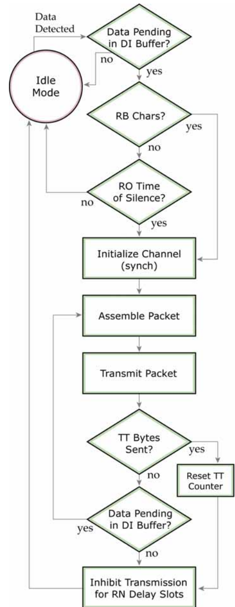
Figure 5-03. Streaming Mode State Diagram
