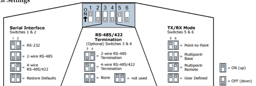
Figure 1-02. DIP Switch Settings
