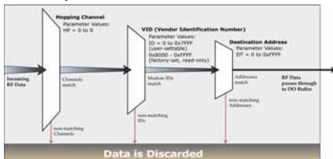
Figure 3-06. Network Layers Contained in the Header
