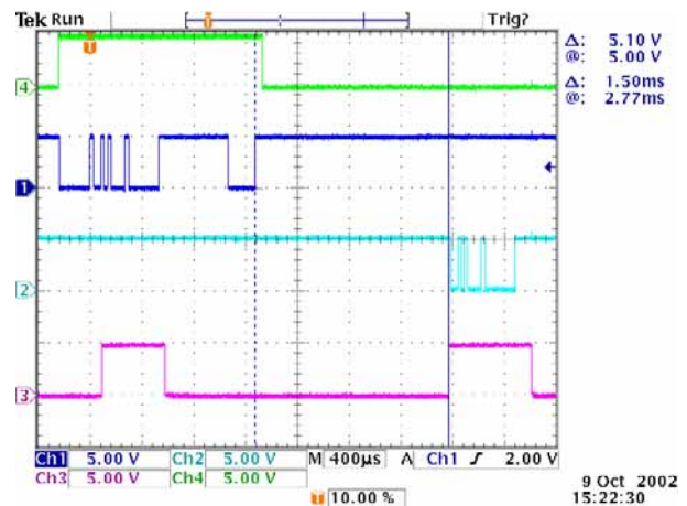
Figure 3-09. Binary Command Write then Read Signal #4 is CMD Signal #1 is the DIN signal to the modem Signal #2 is the DOUT signal from the modem Signal #3 is \overline{CTS}
