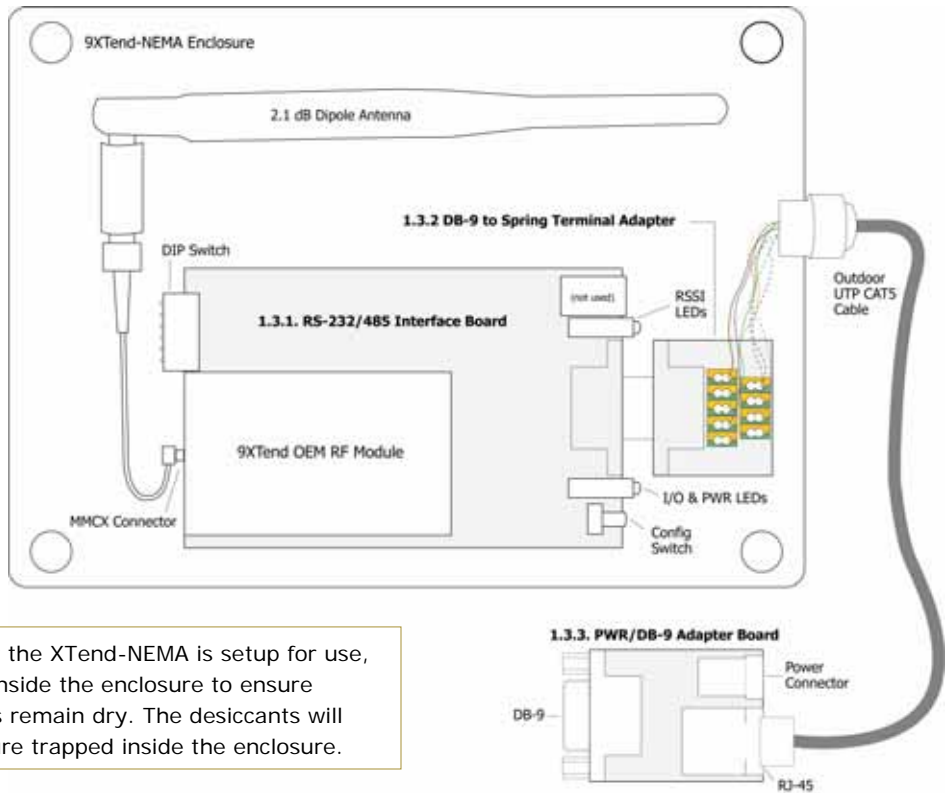
Figure 1-01. Internal Components of the XTend-NEMA RF Modem
