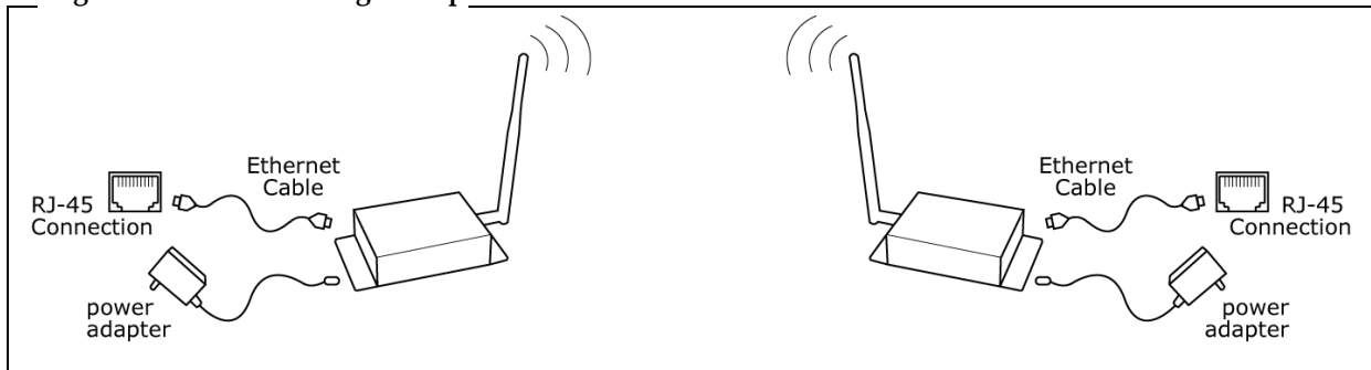
Figure 1. Ethernet Bridge Setup
