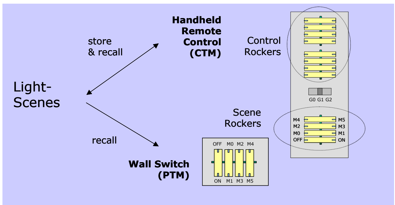
Figure 10: Principle of RCM 110 Scene Selection Control
