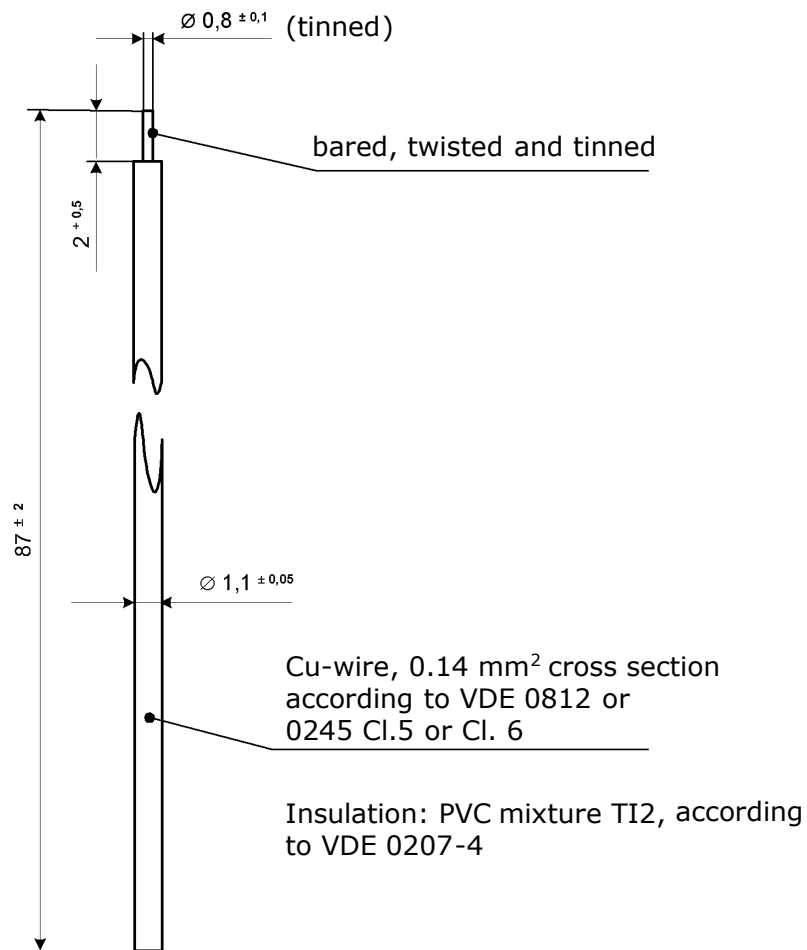
Figure 13: Specification of the RCM whip antenna
